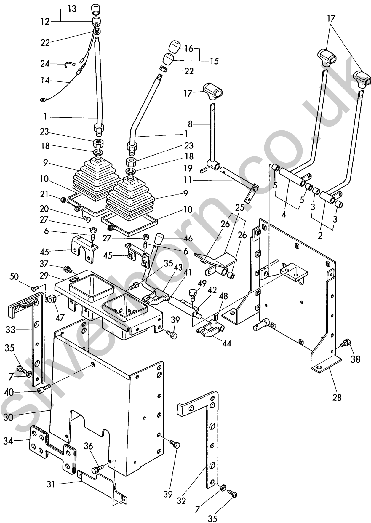
Fig. 18 ソウジュウソウチ(レバー)(キュウガタ) CONTROL EQUIPMENT (LEVER) (PREVIOUS) (YB121U: M/ #00698マデ) (YB151U: M/ #00608マデ) (YB121U: TO M/ #00698) (YB151U: TO M/ #00608)
