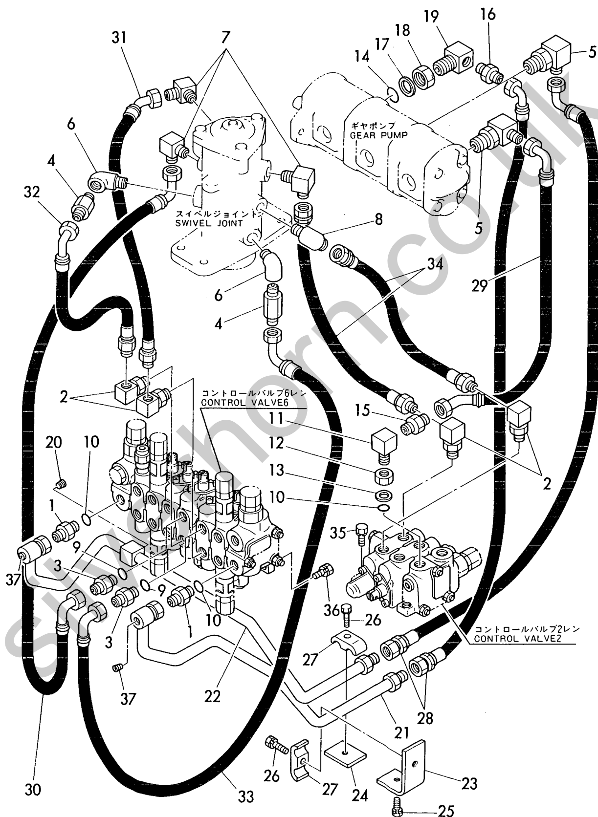
Fig. 34 ユアツハイカン(バルブスイベル)(キューガタ) HYD. OIL PIPING (VALVE-SWIVEL) (PREVIOUS) (YB121U: M/ #00698マデ) (YB151U: M/ #00608マデ) (YB121U: TO M/ #00698) (YB151U: TO M/ #00608)
