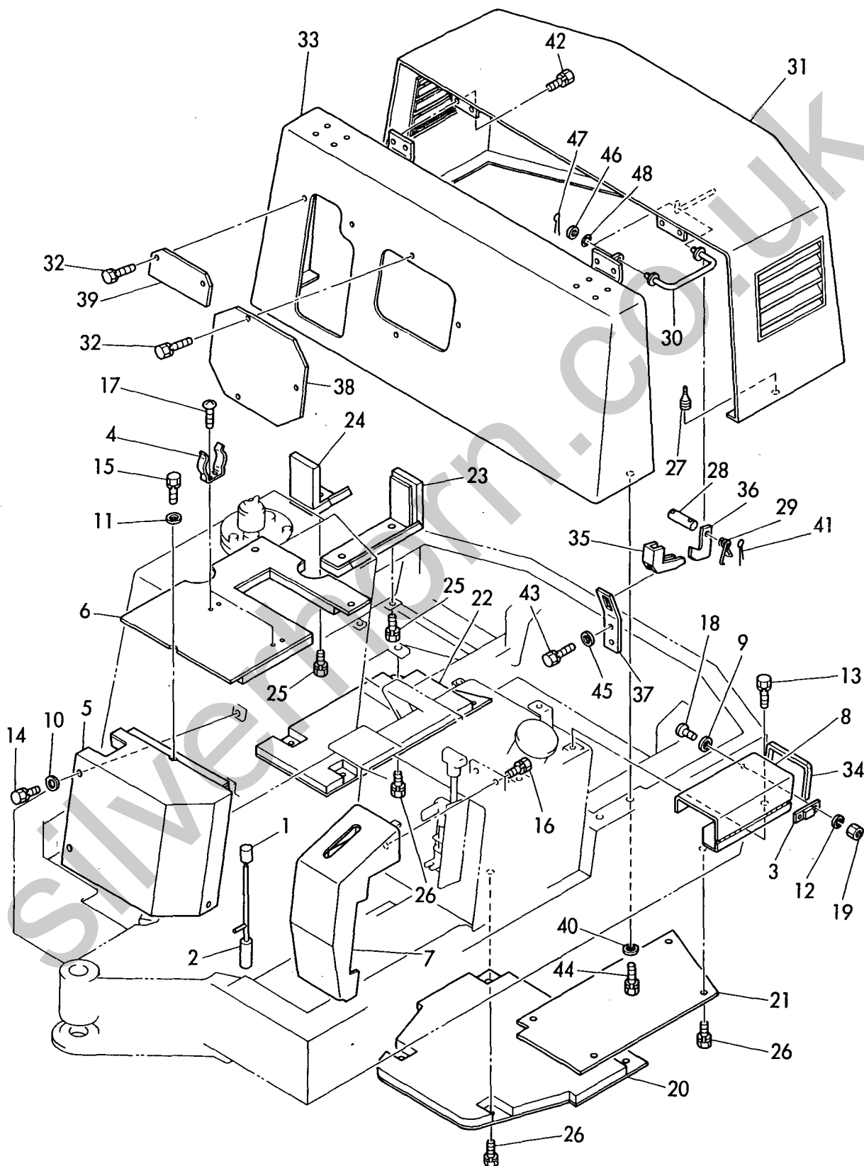
Fig. 25 ボンネット(キューガタ) BONNET (PREVIOUS) (YB121U: M/ #00698マデ) (YB151U: M/ #00608マデ) (YB121U: TO M/ #00698) (YB151U: TO M/ #00608)
