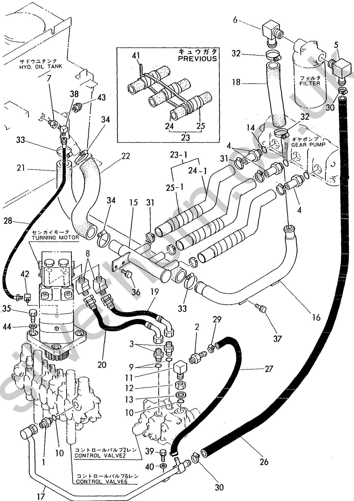
Fig. 37 ユアツハイカン(タンクーバルブモータ)(シンガタ) HYD. OIL PIPING (TANK-VALVE-MOTOR)(NEW TYPE) (YB121U,YB151U: M/ #10501カラ) (YB121U,YB151U: FROM M/ #10501)
